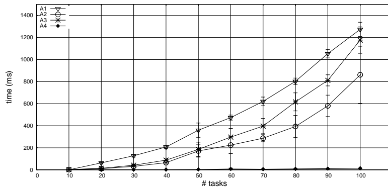
Fig. 9. Execution times for up to 100 tasks on 64 processors
